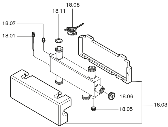
WHW 4
