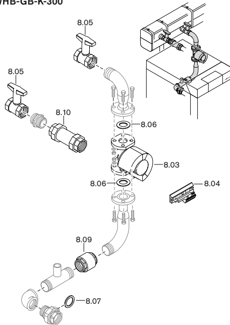
WHB-GB-K-300
