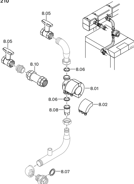
WHB-GB-K-300
